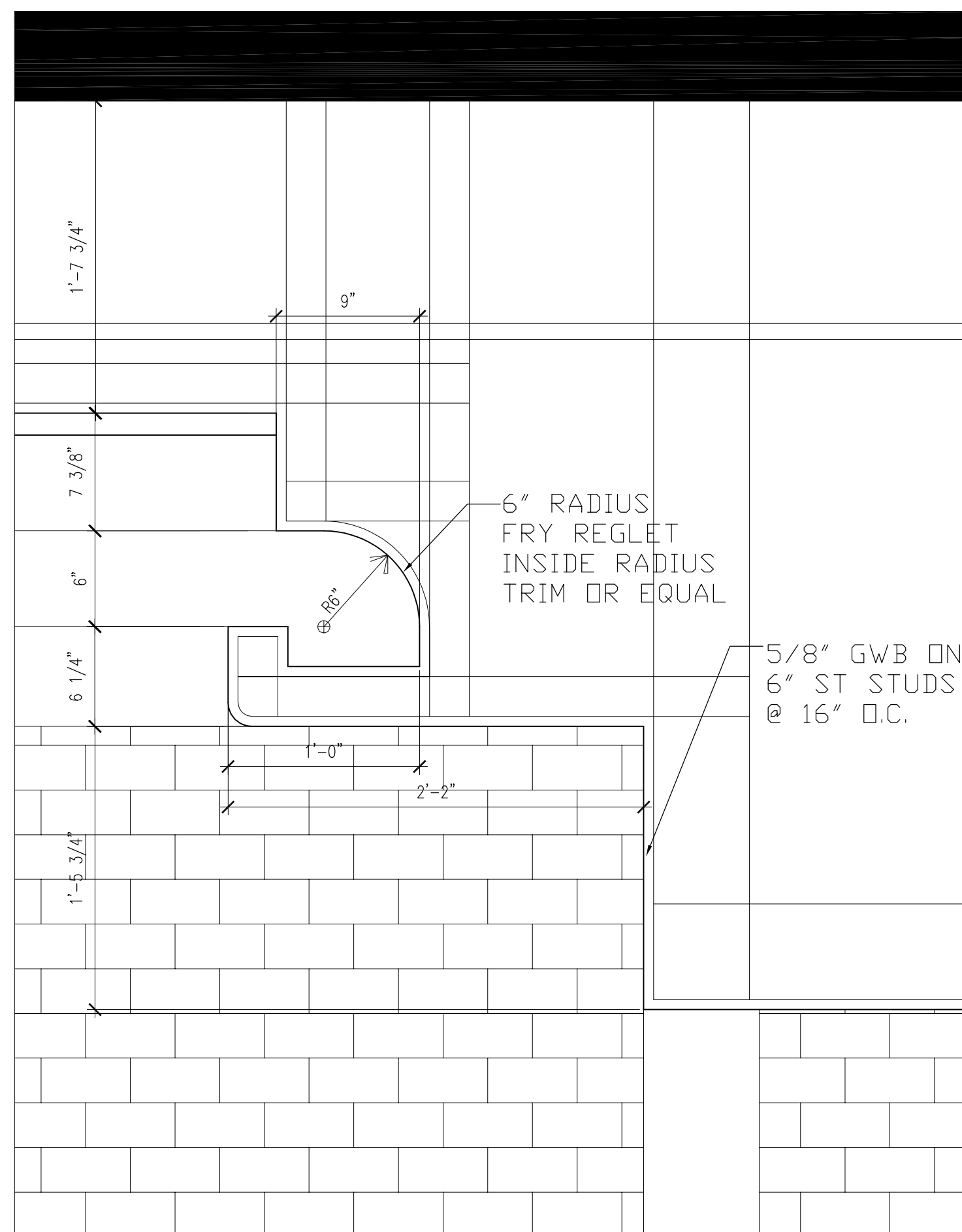
4 CEILING SECTION DETAIL A-102.2 SCALE: 1-1/2" = 1'-0"
