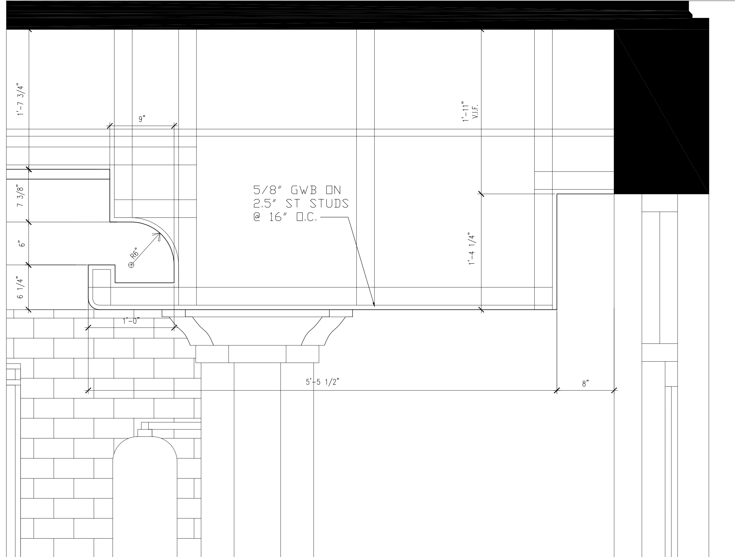
3 CEILING SECTION DETAIL A-102.2 SCALE: 1-1/2" = 1'-0"
