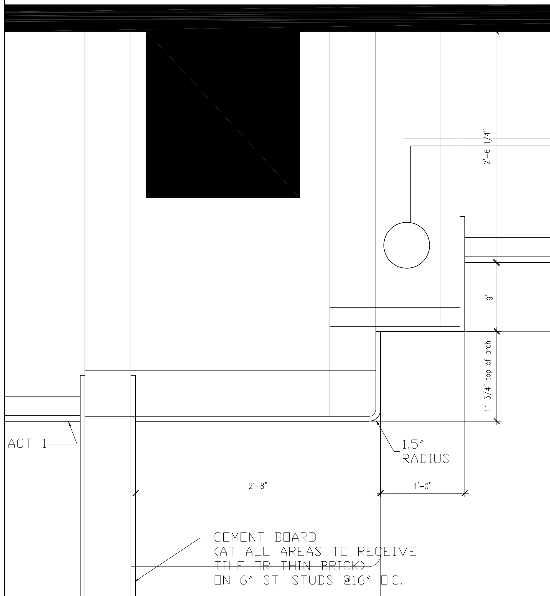
1 CEILING SECTION DETAIL A-102.2 SCALE: 1-1/2" = 1'-0"
