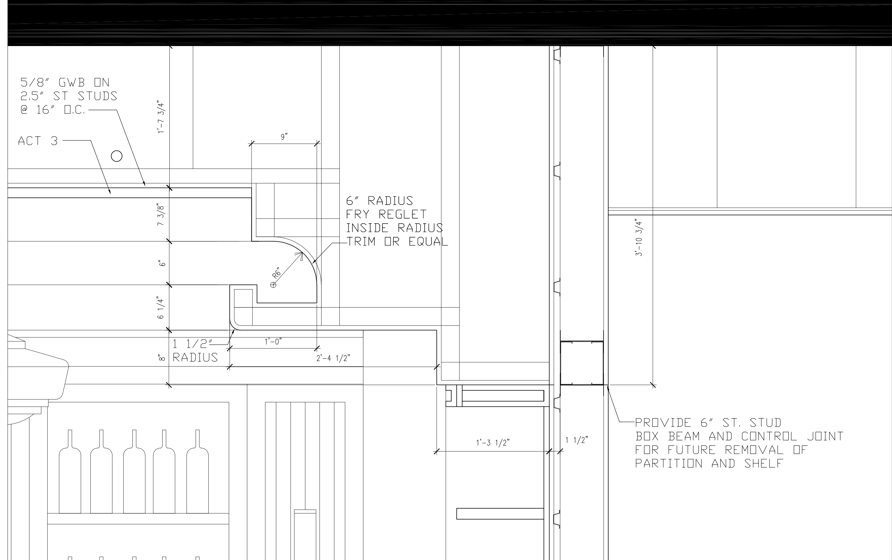
6 CEILING SECTION DETAIL A-102.2 SCALE: 1-1/2" = 1'-0"
