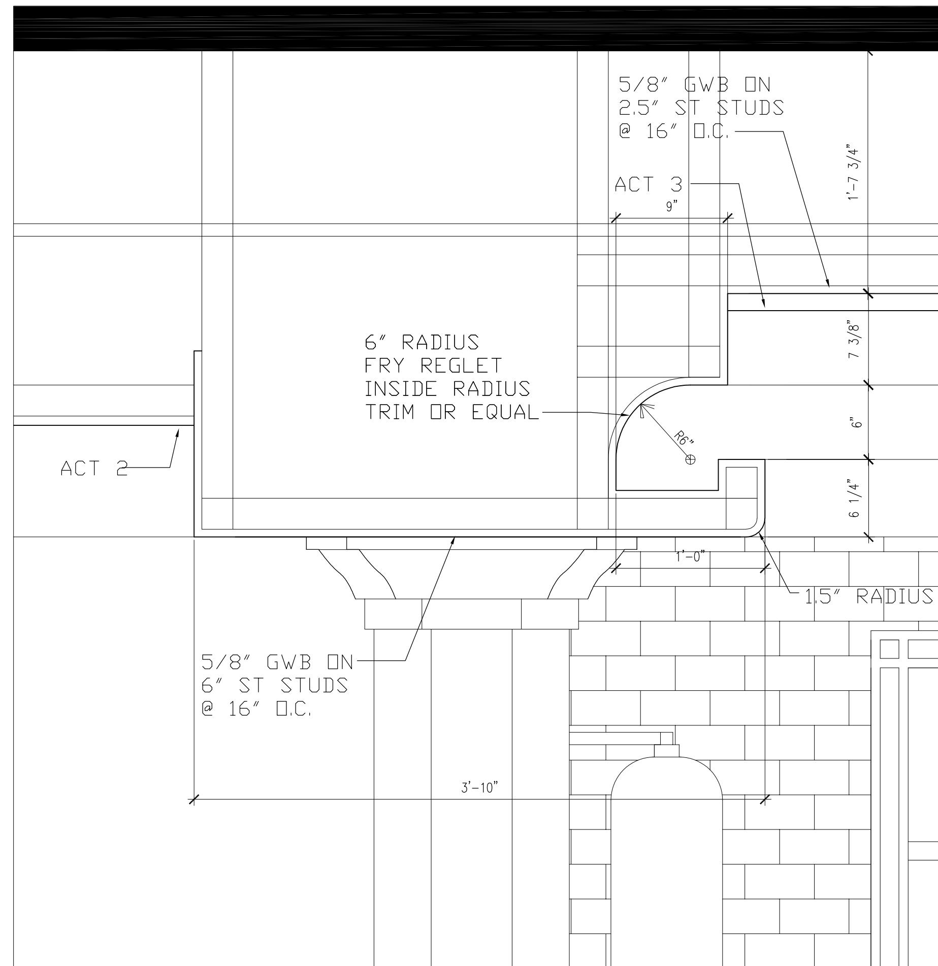
2 CEILING SECTION DETAIL A-102.2 SCALE: 1-1/2" = 1'-0"
