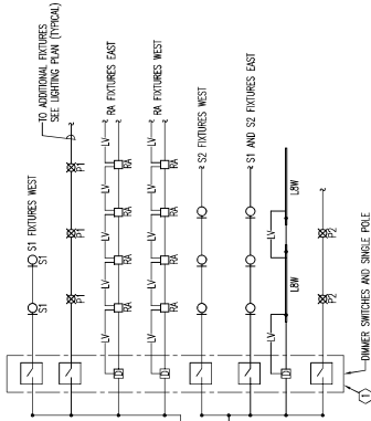
FOOD HALL LIGHTING SEATING AREA LIGHTING CONTROLS
